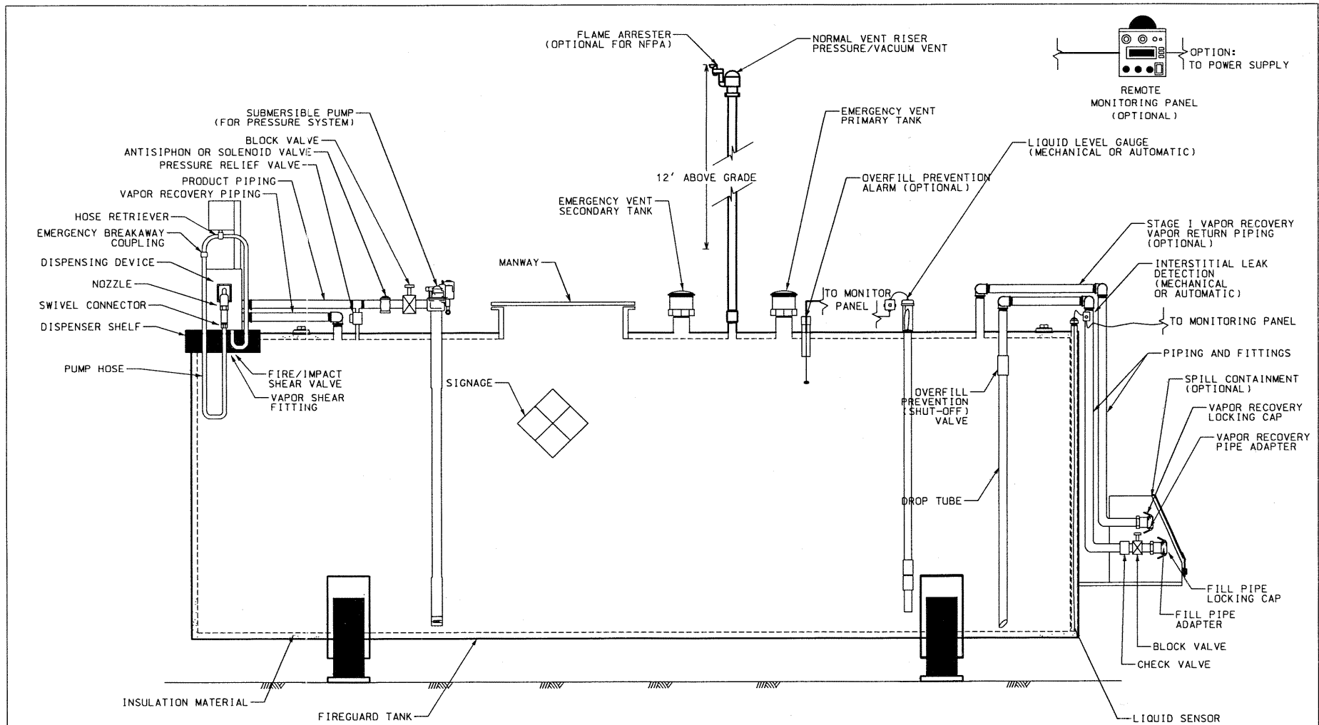
ETHANOL MOTOR VEHICLE FUEL DISPENSING SYSTEM
